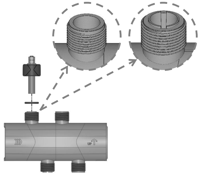
Probe (pH or ORP) with probe holder
